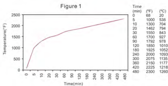
▲ Fire Exposure Test - ASTM E152 Time-Temperature Curve.
